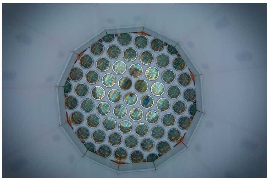
LUX Dark Matter
