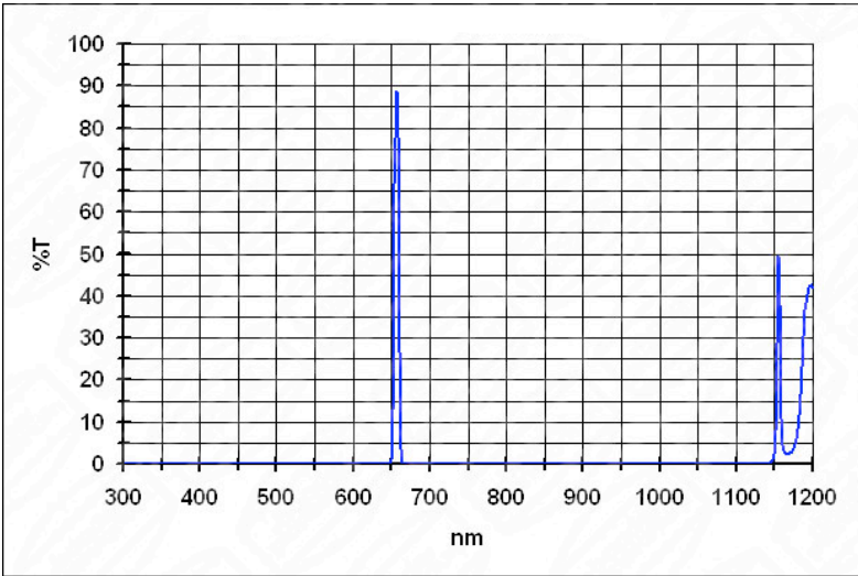
H- \alpha
