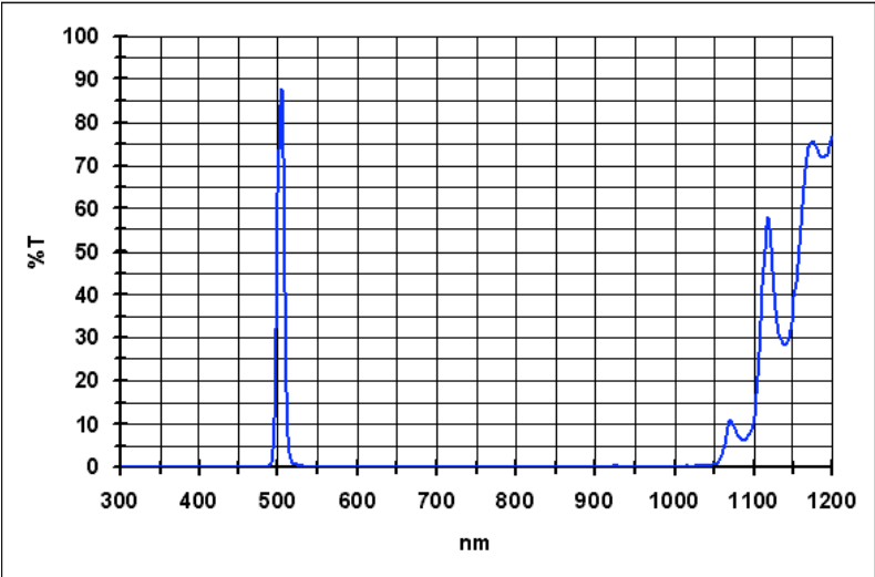
O-III
